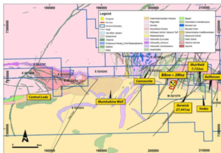
Figure 12. Karlawinda current near mine exploration targets
