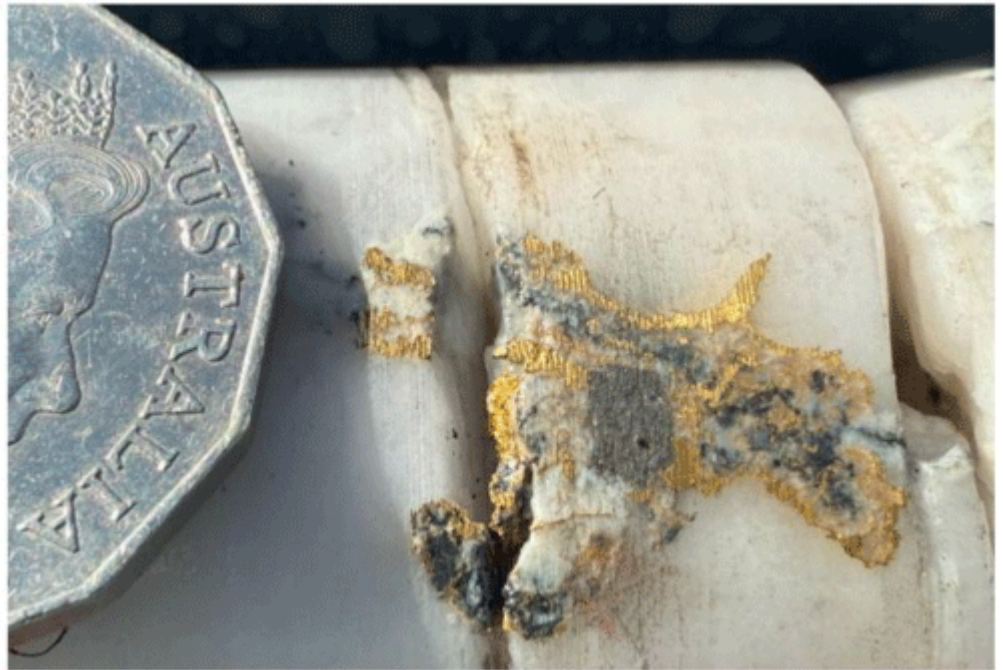
Figure 1 Visible gold in BMDD001W1 at 544.6m depth
