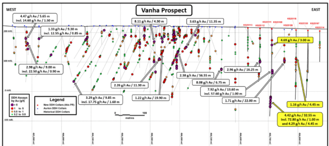
Figure 3: Schematic long section (looking north) of the Vanha prospect, Kaarelseleä area, Risti property.
